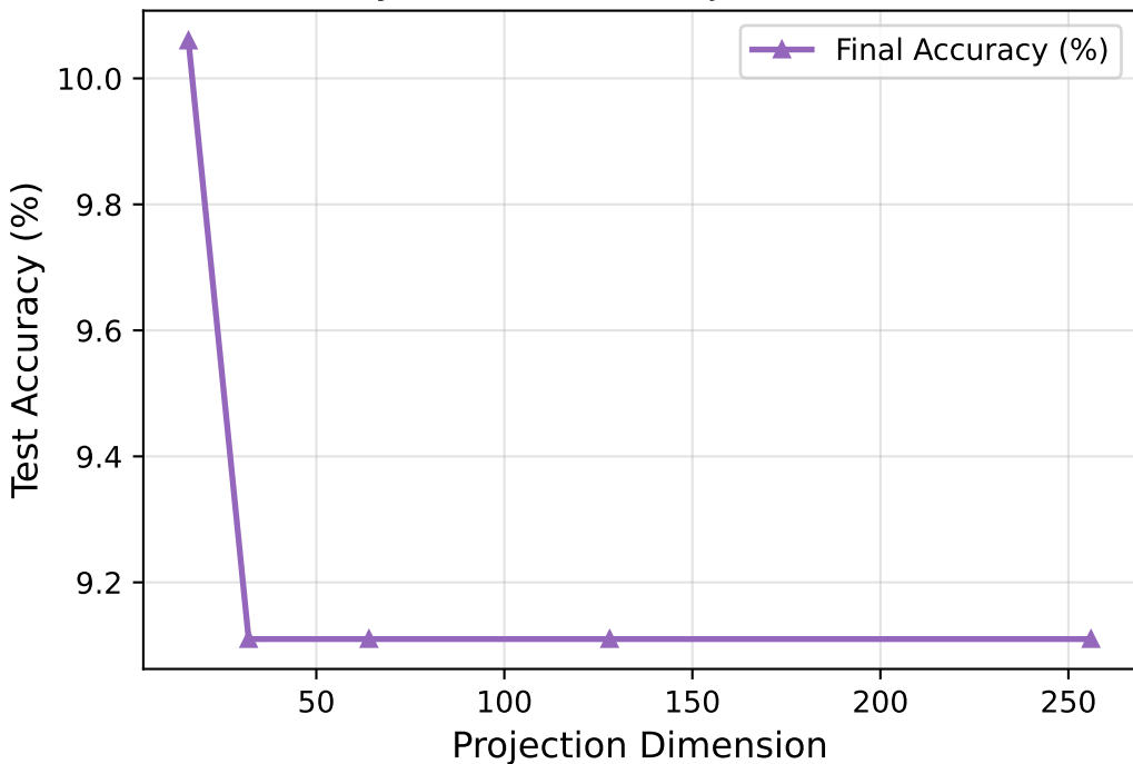
Accuracy vs. Random Projection Dimension
