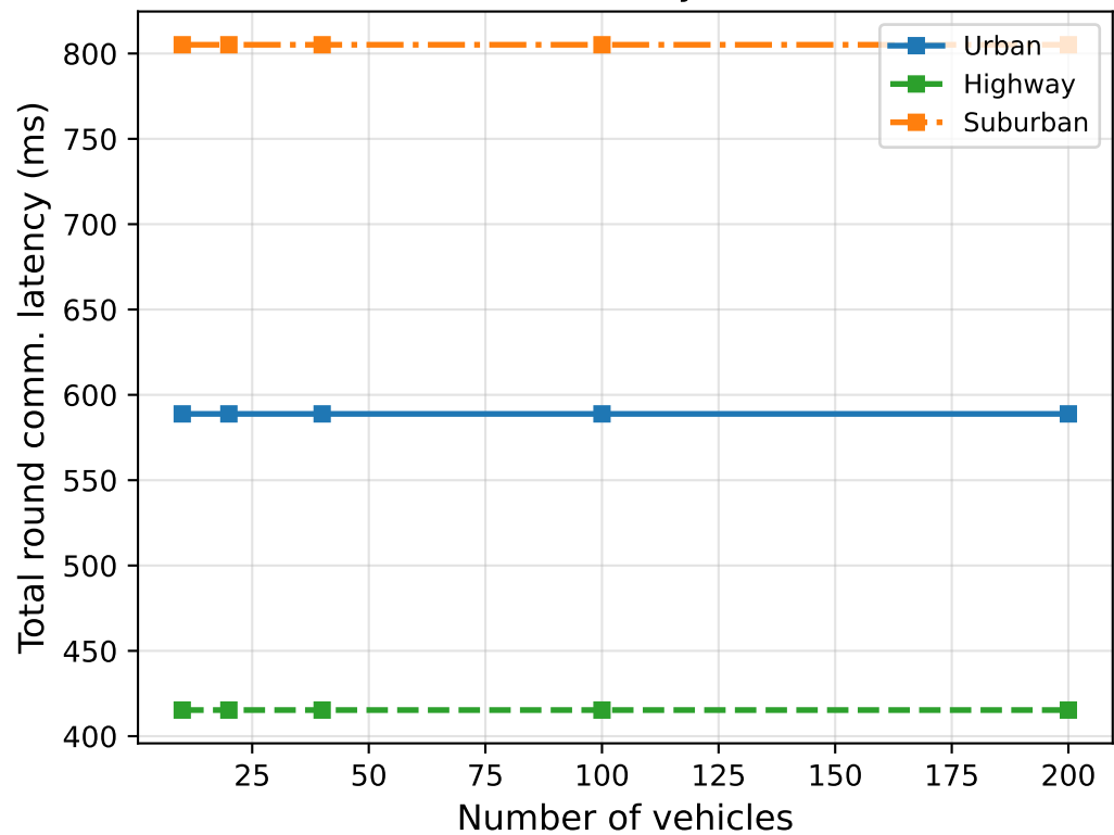
End-to-End Latency vs Vehicles
