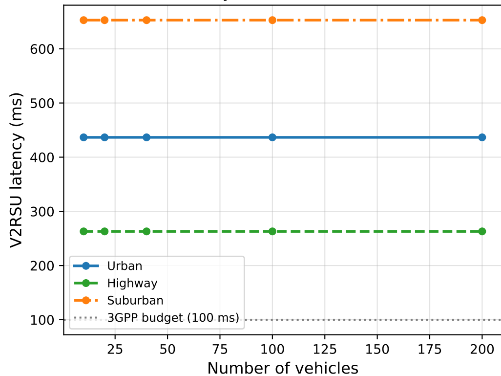
V2RSU Latency vs Vehicles (3GPP NR-V2X)
