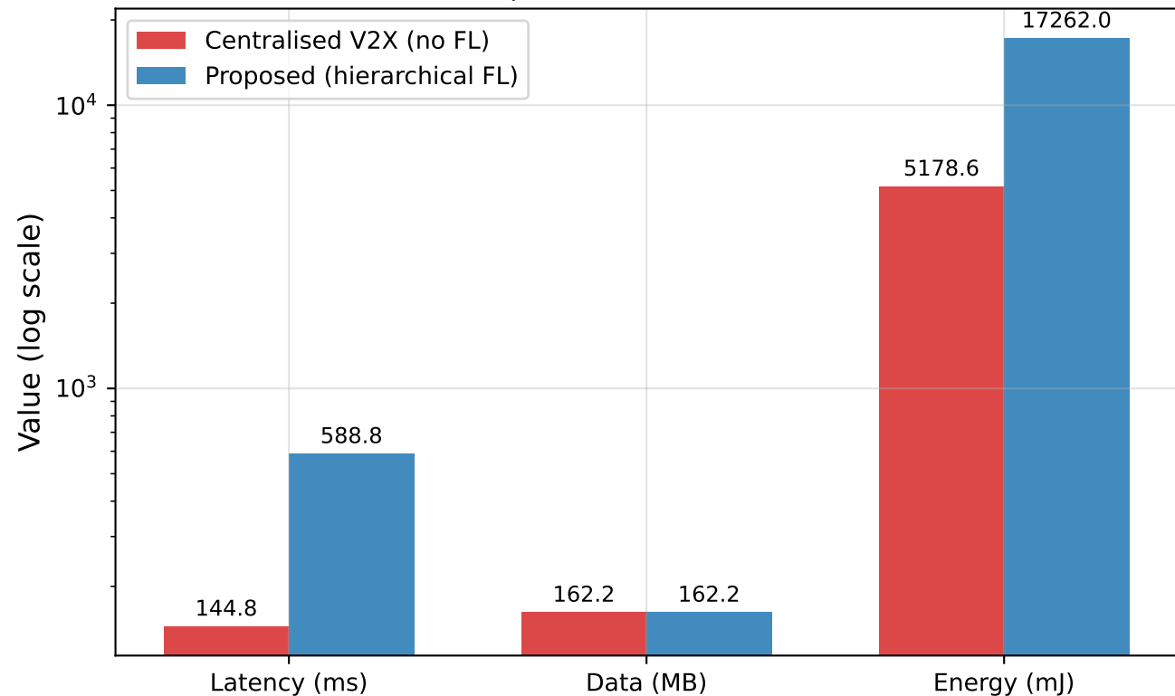
Centralised V2X vs Proposed FL (200 vehicles, Urban scenario)
