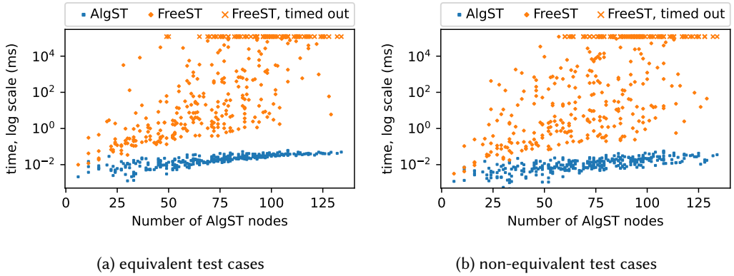
Fig. 12. Execution time of the AlgST and FreeST type equivalence algorithms on the equivalent and non-equivalent test cases, represented in log scale as a function of the number of AlgST nodes in the AST.
