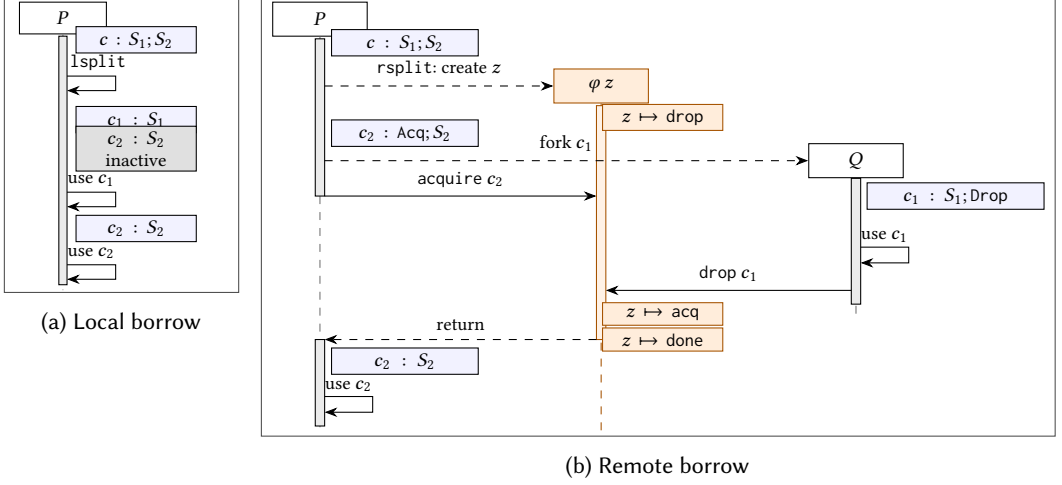
Fig. 3. Message-sequence view of local and remote borrows. Channel state is shown as annotations next to the relevant process or flag lifelines. A local split keeps the channel state with the original process lifeline; a remote split creates a flag lifeline \phi z and forks a process for the borrowed prefix.
