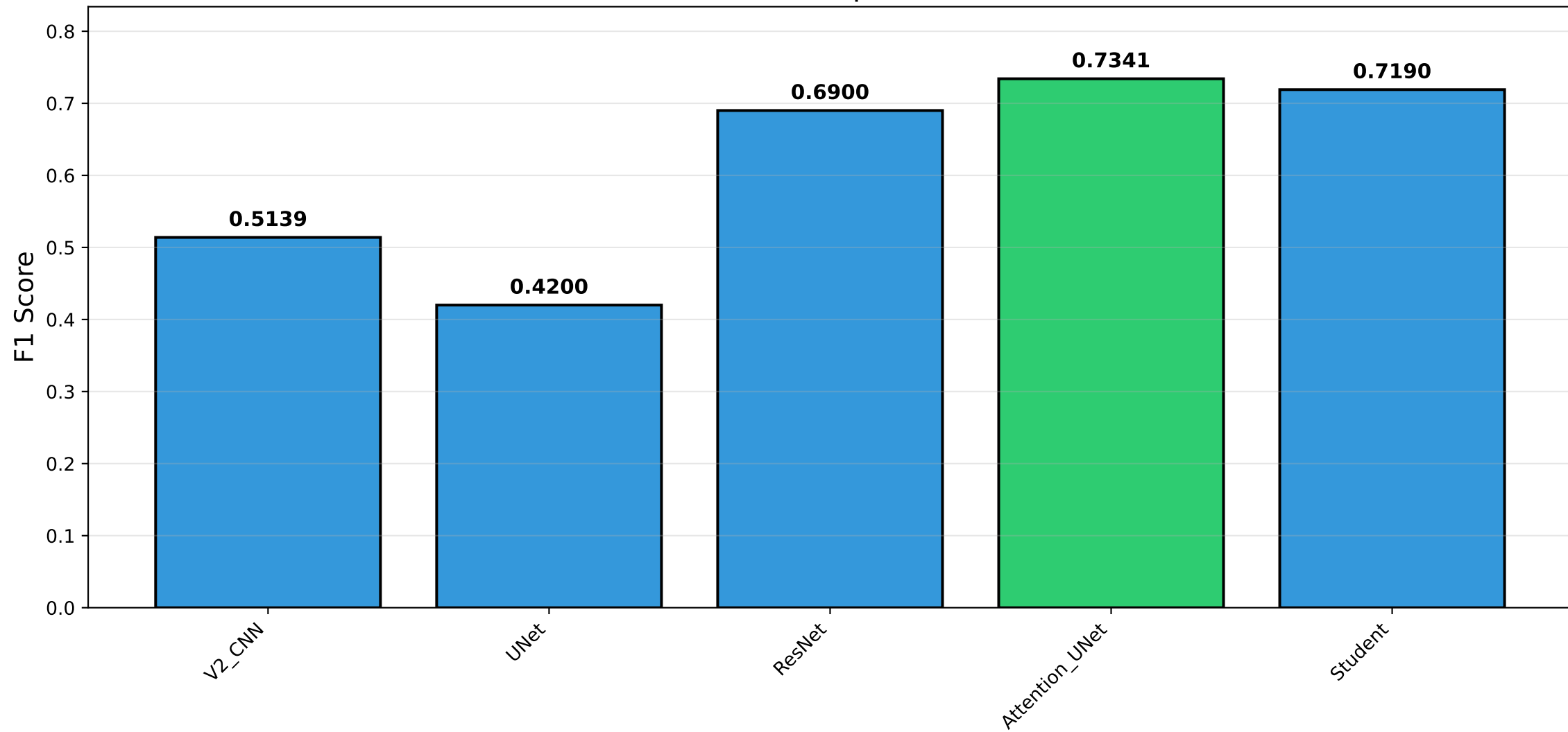
Model Performance Comparison - All 5 Models
