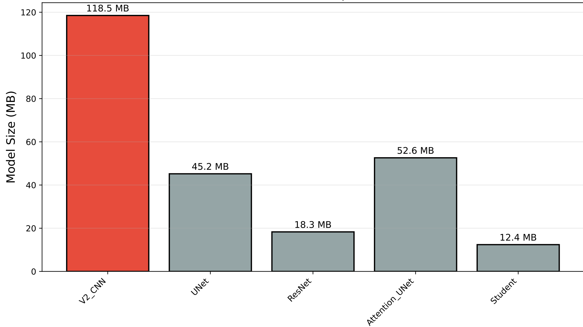
Model Size Comparison
