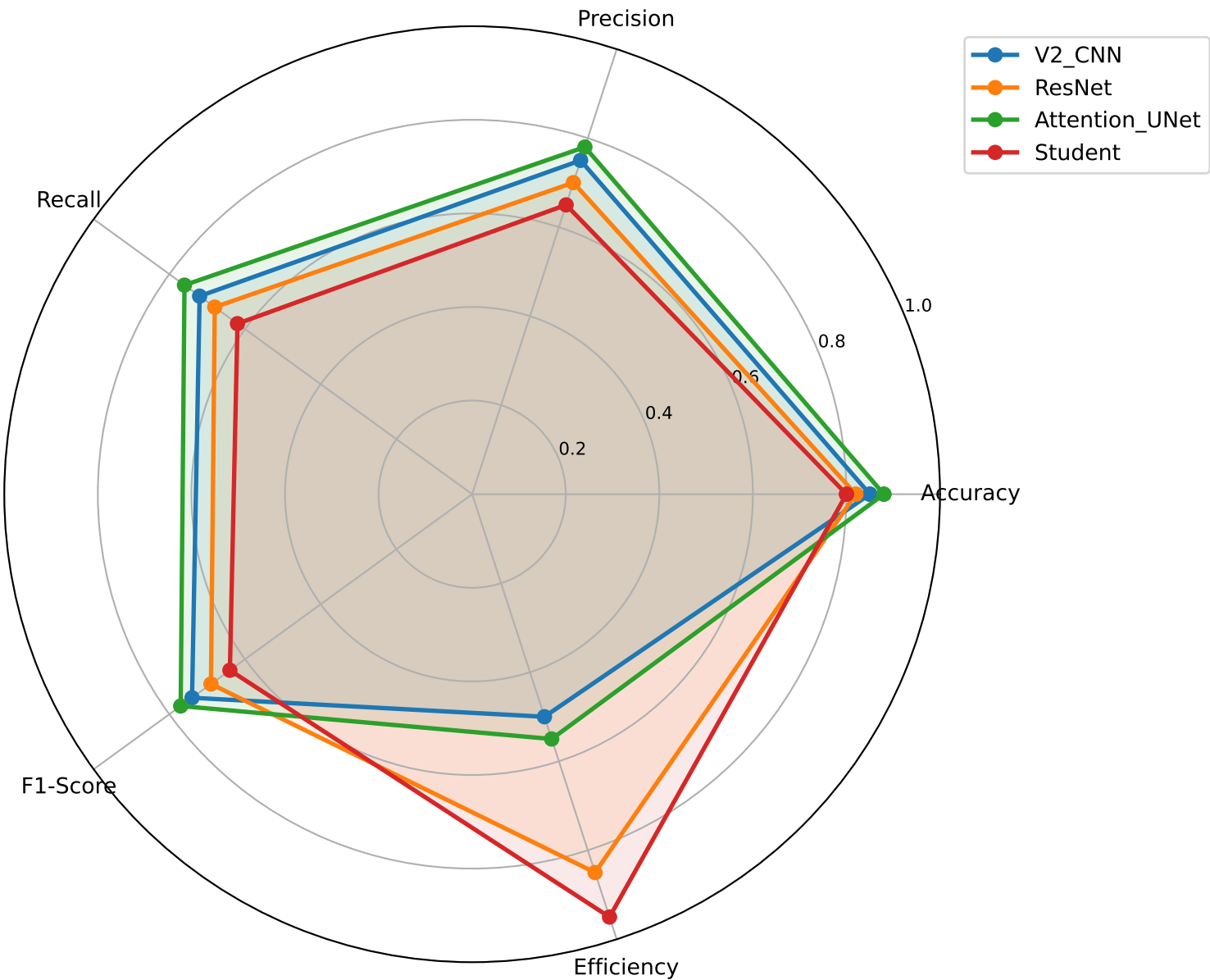
Model Performance Radar Chart
