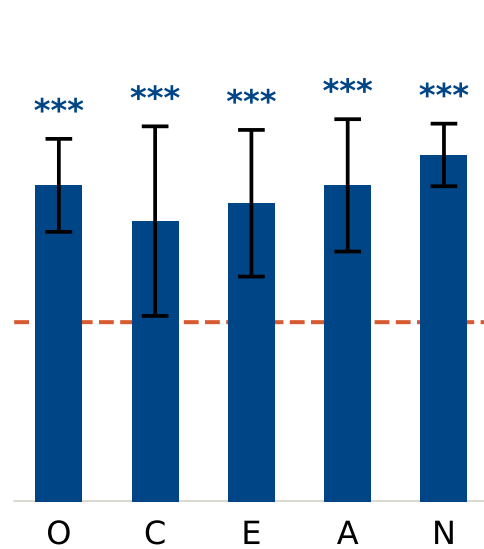
(b) Consistency
