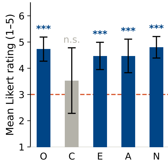
(a) Distinguishability
