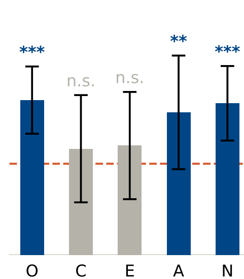
(c) Engagement
