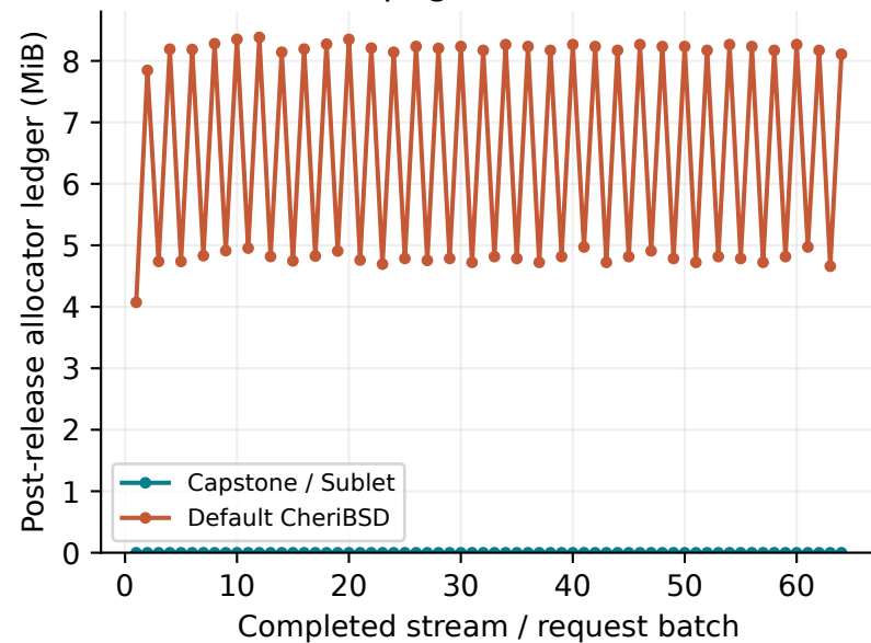
FFmpeg: 64 streams
