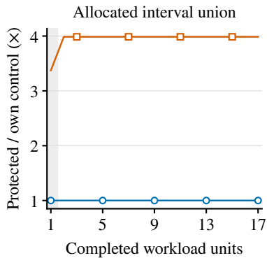
(b) Address coverage
