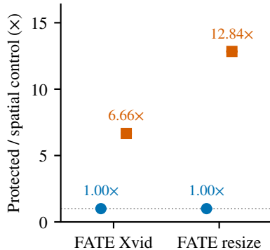
(c) FFmpeg pool Carved address extent
