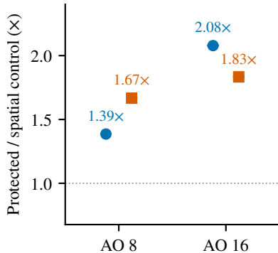
(b) GC backing After render
