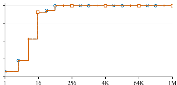
(h) FFmpeg · pool leases 16 × 30-frame stream
