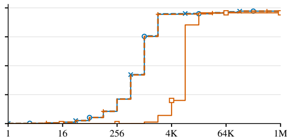
(b) mruby · GC slots AO, width 8
