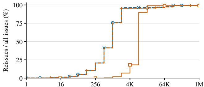
(c) mruby · GC slots AO, width 16
