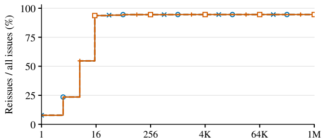
(e) FFmpeg · pool leases FATE resize, 150 frames
