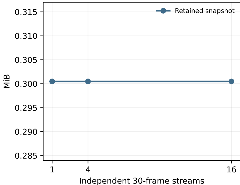
Snapshot backing persists across streams
