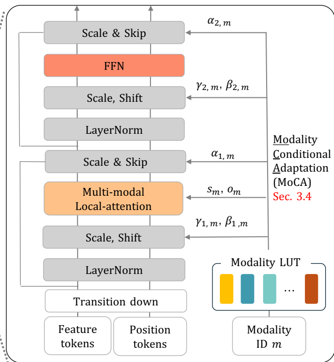
(b) Universal Encoder Block
