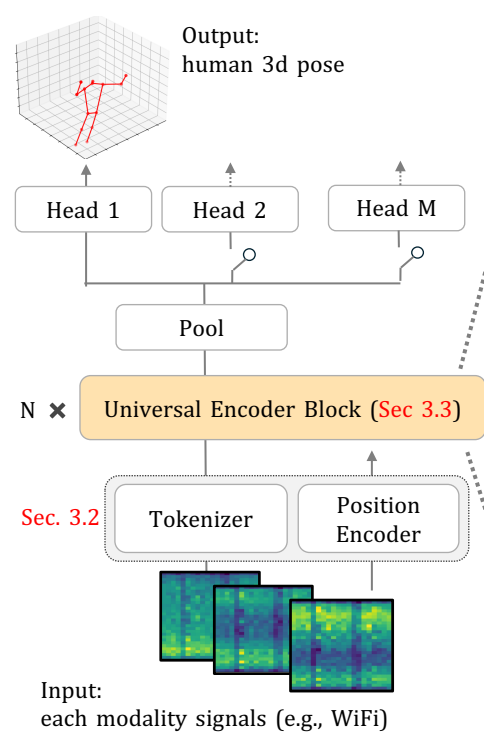
(a) Universal Transformer
