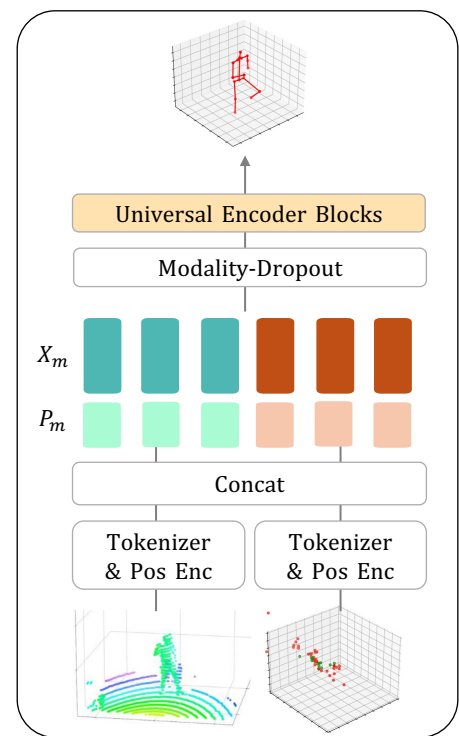
(c) Multi-modal fusion (Sec 3.5)
