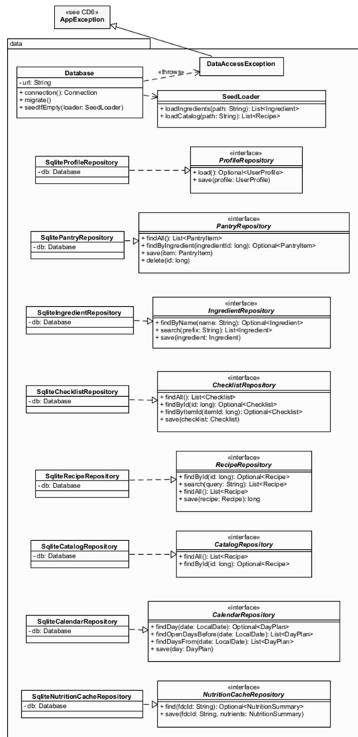
CD7 · Persistence (package data): Repository interfaces over SQLite
