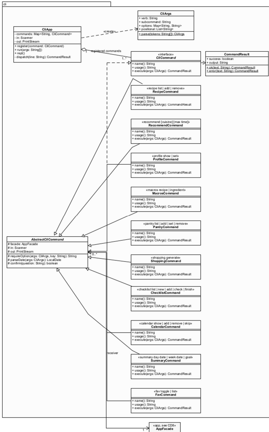
CD9 - Command-line interface (package cli): Command pattern
