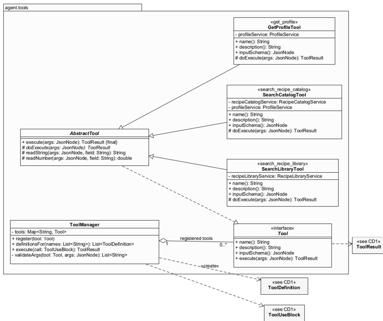
CD2 · Agent tools (package agent.tools): Template Method + registry
