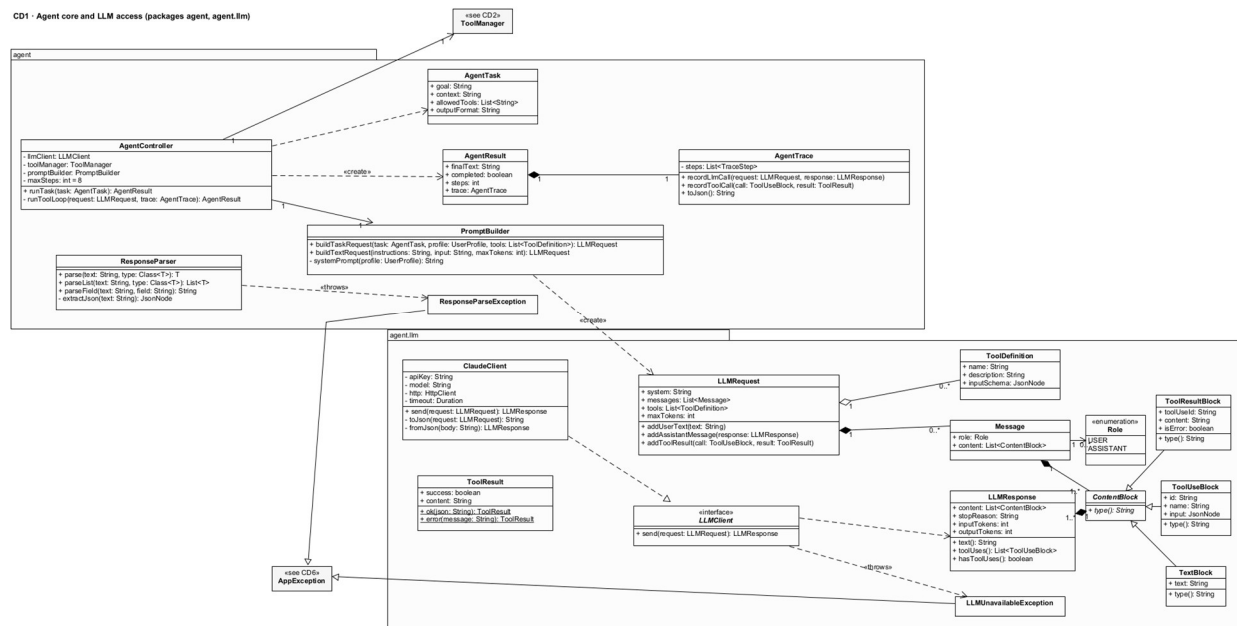
CD1 - Agent core and LLM access (packages agent, agent.llm)
