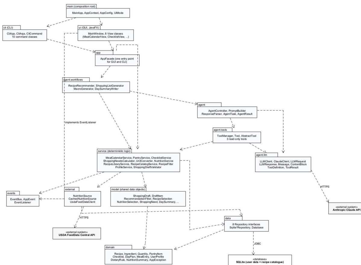
Overall Architecture: packages and their dependencies
