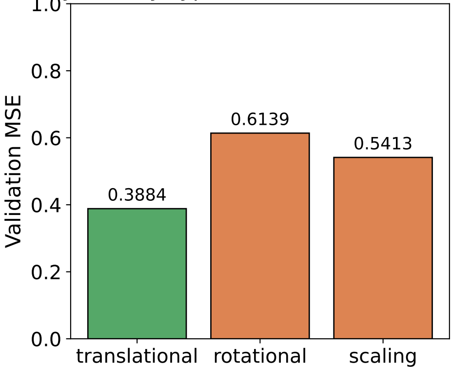
Symmetry Type (winner: translational)
