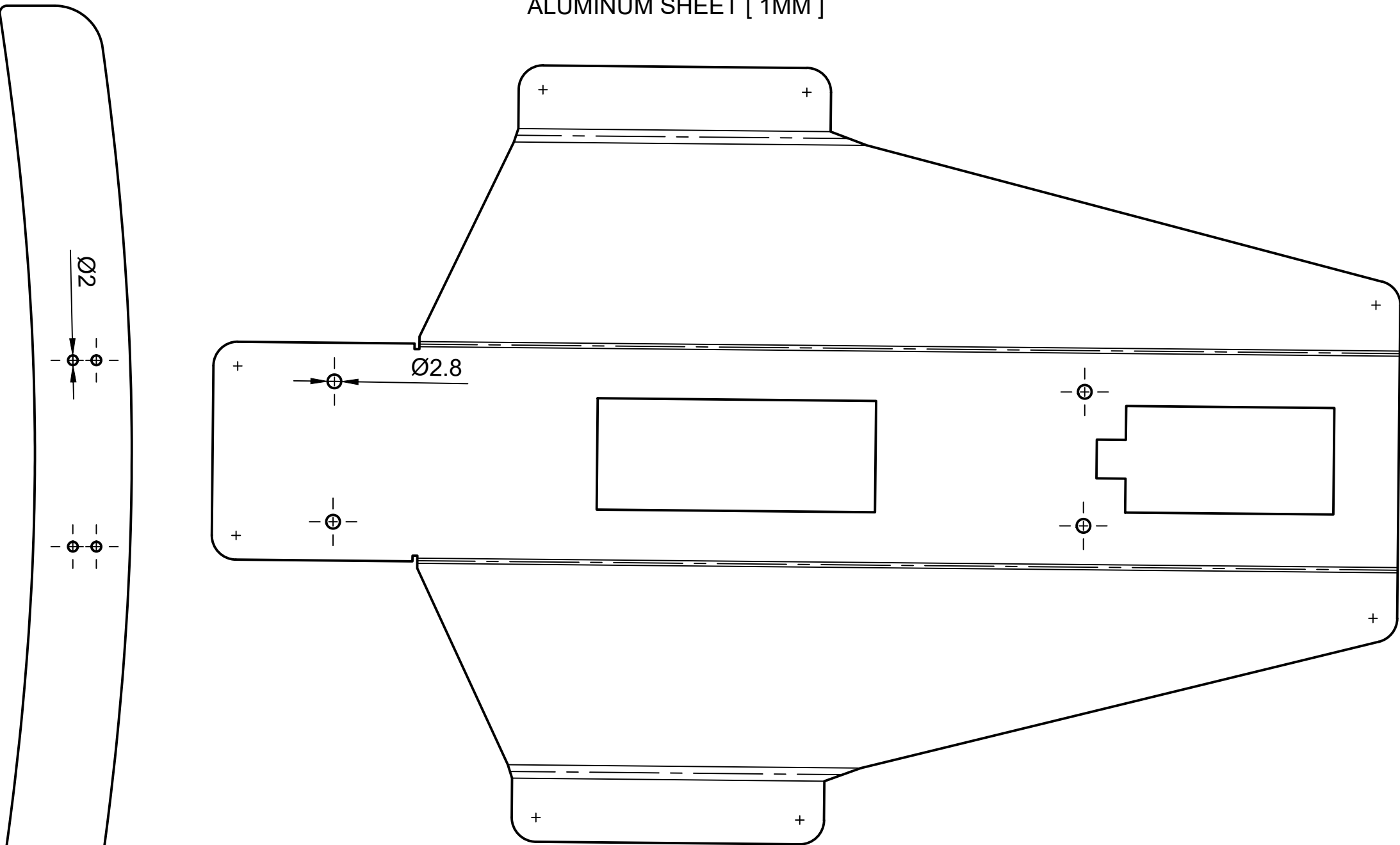
ALUMINUM SHEET [ 1MM ]
