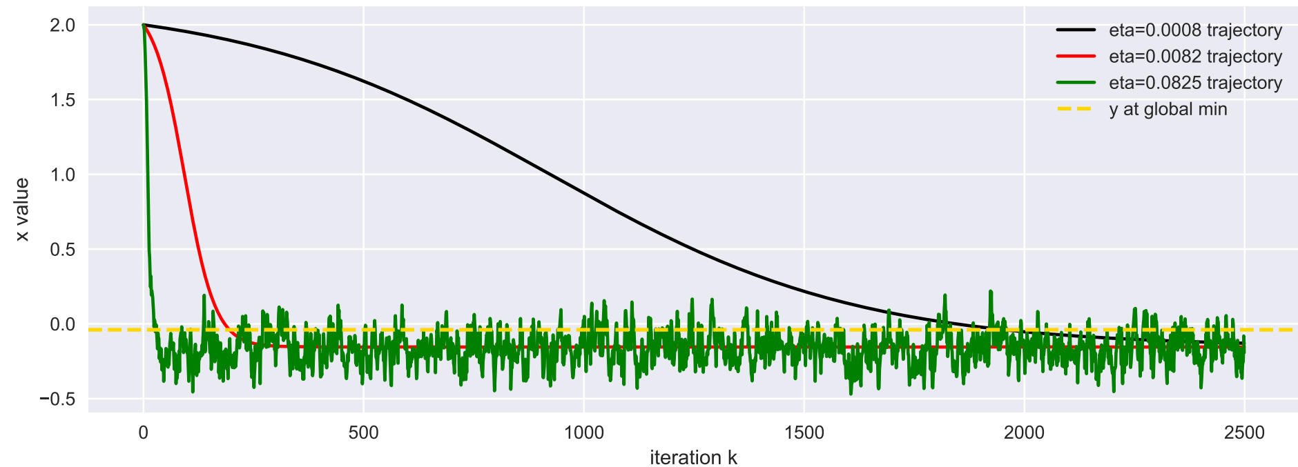
SGD: x vs Iterations
