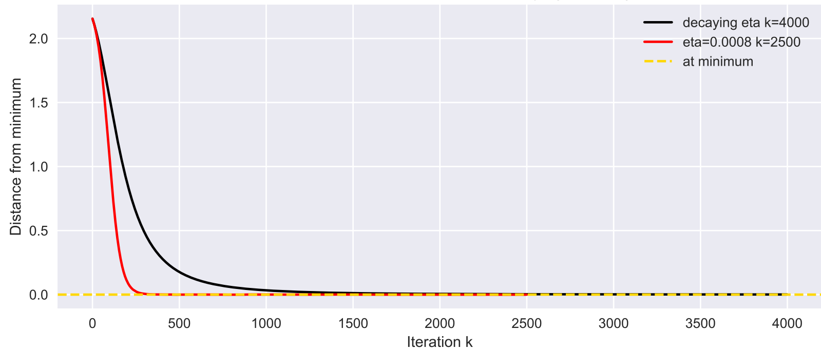
SGD: Distance from min - Constant Vs Decaying Learning Rate
