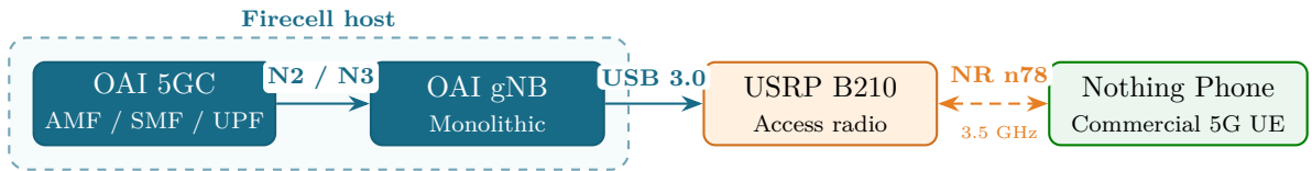
Figure 1: Monolithic OAI 5G SA Reference Architecture
