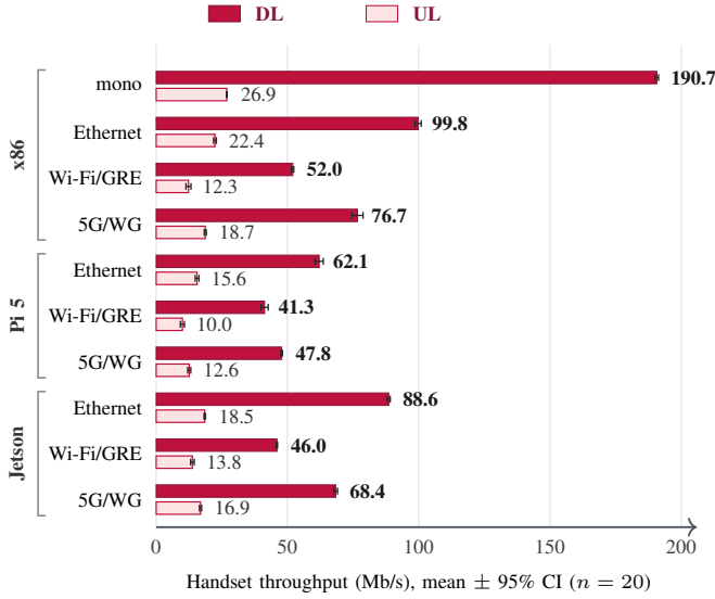
Fig. 2. Mean handset Downlink (DL, solid) and Uplink (UL, light) throughput across all 10 configurations ( n = 20 per setup, 400 total observations).
