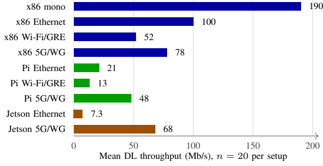
Fig. 2. Mean handset downlink over 20 accepted repetitions per setup. The artifact does not retain dispersion, so no error bars are shown.
