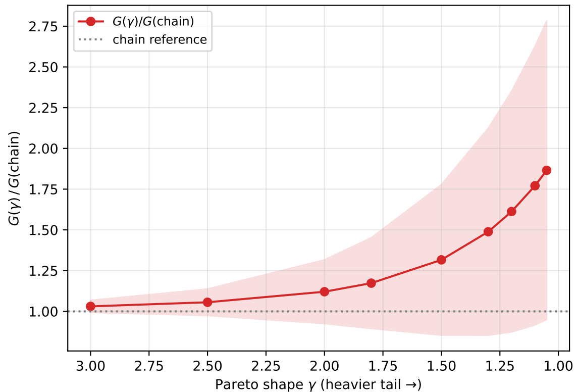
Pareto-shape sweep at M = 50 (mean \pm std, 200 seeds)
