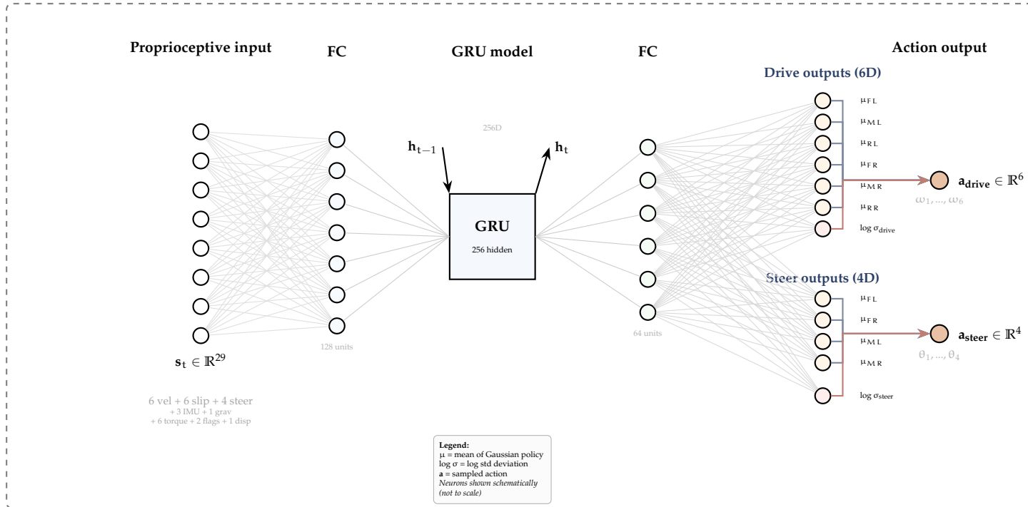
Figure 4: Structure of the Mars rover control policy network. The GRU (256 hidden units) processes 29D proprioceptive features (wheel velocities, slip ratios, steering angles, IMU data, gravity projection, drive torques, entrapment flags, and displacement) and outputs 10D actions: 6 independent drive velocities ( \omega_{FL}, \omega_{ML}, \omega_{RL}, \omega_{FR}, \omega_{MR}, \omega_{RR} ) and 4 steering angles ( \theta_{FL}, \theta_{FR}, \theta_{ML}, \theta_{MR} ). Actions are sampled from Gaussian distributions parameterized by the network. Neurons shown schematically, not to scale.
