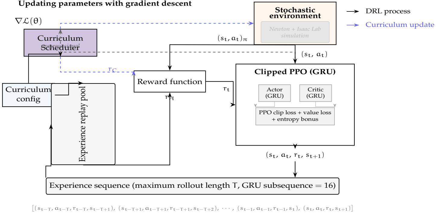
Figure 5: Block diagram of the reward-shaped DRL training loop. The curriculum scheduler (replacing GAIL’s discriminator) adjusts sinkage depth and reward weights based on training progress. Shaped reward r_t = r_H (hand-crafted) combines progress, escape milestones, rocking, and penalty terms. The GRU-PPO agent is updated via clipped surrogate loss with entropy bonus.
