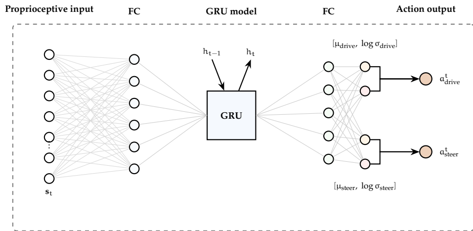
Figure 4: The structure of the Mars rover control policy network. GRU (256 hidden units) processes 29D proprioceptive features and outputs 10D actions (6 drive velocities + 4 steering angles).
