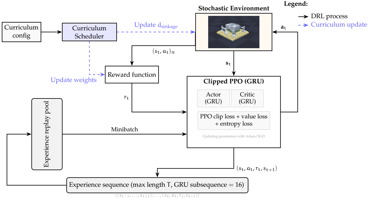
Figure 5: Block diagram of the reward-shaped DRL training loop. The curriculum scheduler updates environment difficulty and reward weights. The closed-loop interaction between PPO and the environment generates transitions, which are stored and sampled as minibatches for policy updates.
