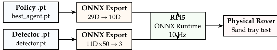
Figure 10: Planned sim-to-real deployment pipeline.
