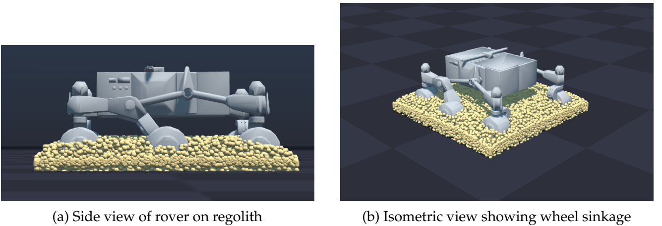
Figure 7: Newton simulation environment showing the AAU 6-wheel Mars rover on granular regolith. The MPM particle bed ( 2.0 \text{ m} \times 2.0 \text{ m} \times 0.15 \text{ m} ) provides realistic sinkage and wheel-sand interaction under Martian gravity ( 3.72 \text{ m/s}^2 ). Screenshots to be captured from Newton ViewerGL.
