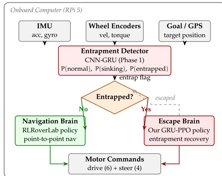
Figure 17: Dual-brain onboard architecture. The CNN-GRU entrapment detector switches control between the RLRoverLab navigation policy (normal traversal) and our GRU-PPO escape policy (entrapment recovery). Both policies share the same motor command interface.
