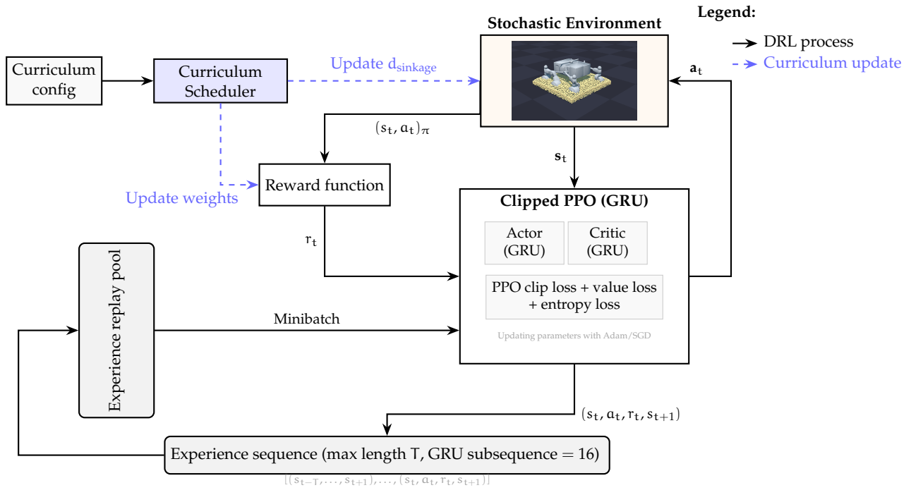
Figure 5: Block diagram of the reward-shaped DRL training loop. The curriculum scheduler updates environment difficulty and reward weights. The closed-loop interaction between PPO and the environment generates transitions, which are stored and sampled as minibatches for policy updates.
