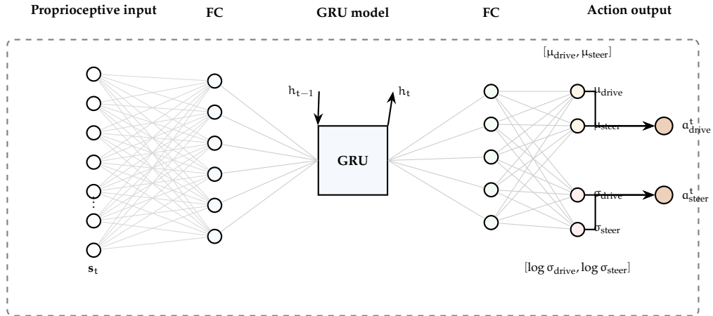
Figure 4: The structure of the Mars rover control policy network (adapted from Bi and Ding [1], Fig. 8). Key differences: LSTM replaced with GRU (256 hidden units, fewer gates); input expanded from 30D to 29D proprioceptive features; output expanded from 2D ( \omega_l, \omega_r ) to 10D (6 drive velocities + 4 steering angles).
