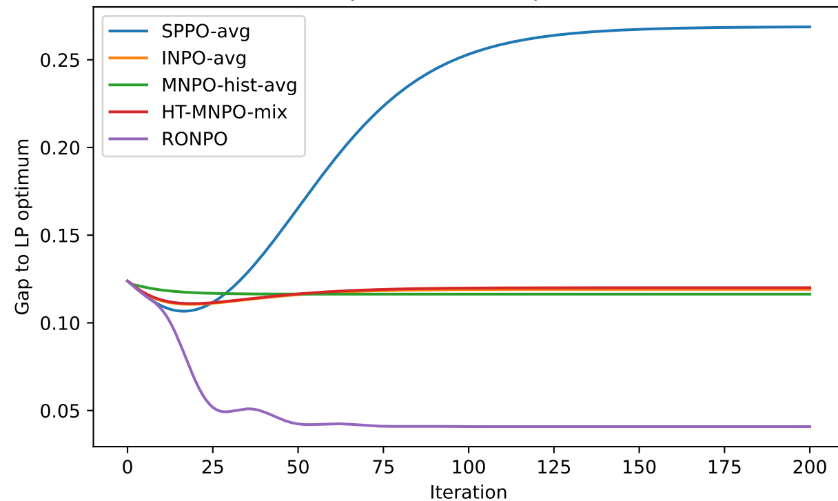
(c) Gap to Robust LP Optimum
