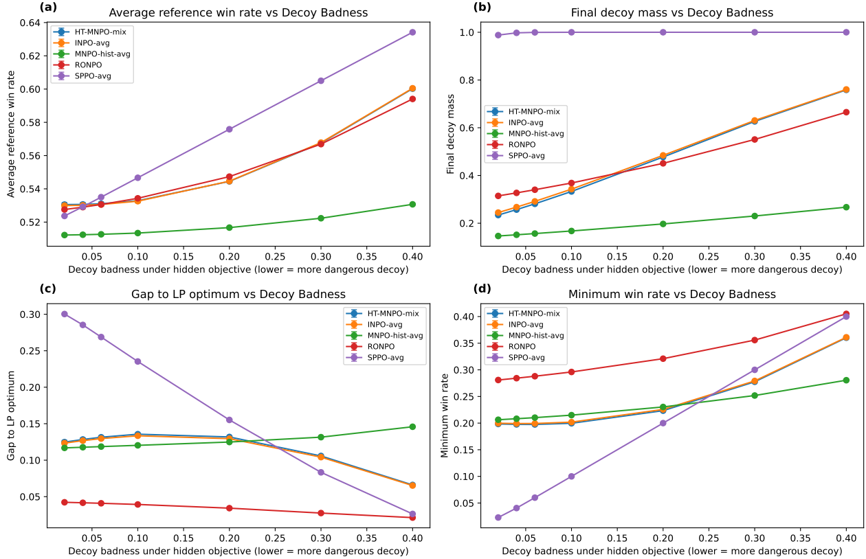
Figure 6: Sweep over the hidden-objective decoy win probability P_3(a_{\text{decoy}} \succ a) . Lower values make the decoy more dangerous. RONPO is most useful in the regime where the averaged oracle masks severe minority-objective failure.
