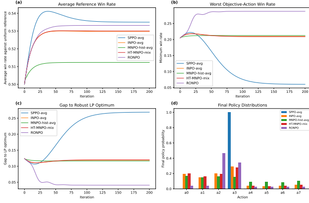
Figure 4: Dynamics over 200 iterations. Averaged-oracle SPPO attains the highest average win rate by collapsing onto the decoy action; RONPO shifts mass toward the robust LP mixture and raises the minimum objective-action win rate.
