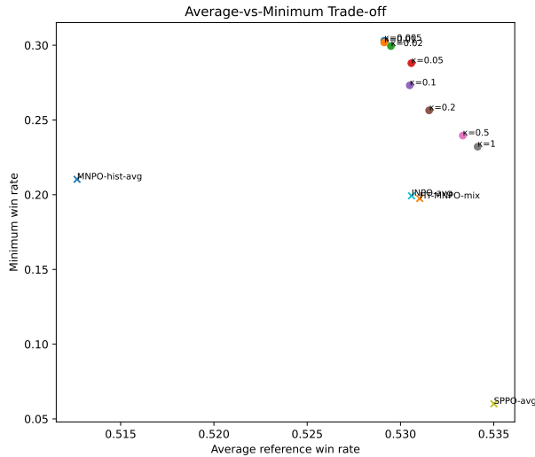
Figure 7: RONPO trade-off as the adversary temperature \kappa varies. Smaller \kappa gives a sharper worst-case adversary; larger \kappa moves toward fixed scalarization.
