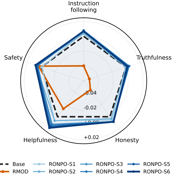
Figure 2: Per-objective raw-reward change from Base on a fresh, prompt-disjoint 647-prompt UltraFeedback panel. The dashed black polygon is the zero-change Base, and RMOD uses K = 16 candidates per block. RONPO stages 1–4 use the stronger-signal pool, while stages 5–6 add the moving anchor. Every response is scored together by the same five ArmoRM heads in one BF16 context. From stage 3 onward, all five RONPO point estimates exceed both Base and RMOD. Results use seed 42, with no reward-based stage selection.
