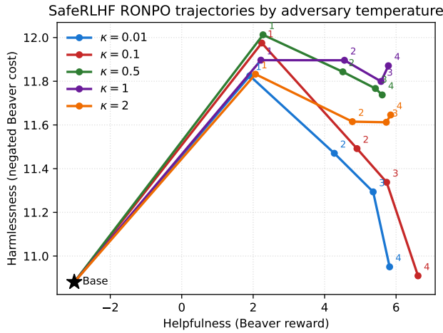
Figure 3: SafeRLHF helpfulness and harmlessness trajectories, measured by Beaver reward and negated Beaver cost on 1,000 held-out prompts. A single Llama-3.1-8B-Instruct Base point anchors the RONPO paths for \kappa \in \{0.01, 0.1, 0.5, 1, 2\} ; the labels mark stages 1–4. All displayed points use one common reward-scoring pass. Connecting lines show the measured stagewise paths and do not assert theoretical monotonicity.
