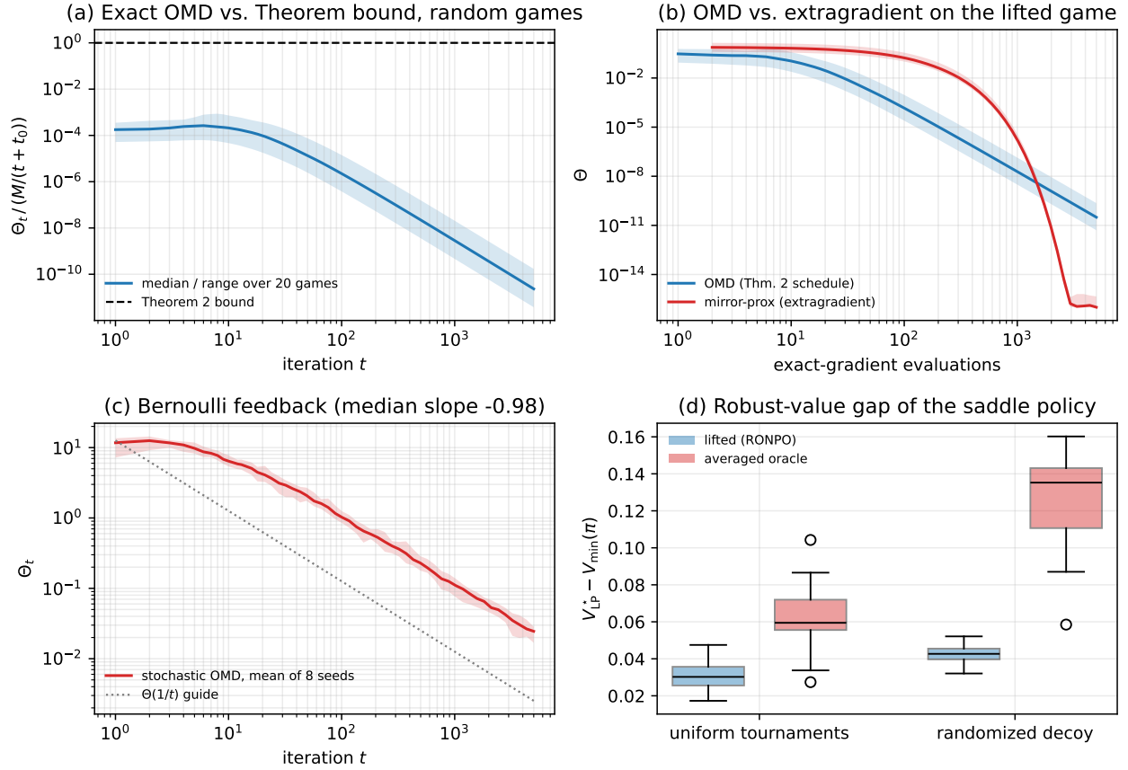
Figure 5: Validation across random game families (20 games per configuration; bands span the min–max range across games, lines are medians). (a) Exact-OMD Lyapunov value relative to the Theorem 2 bound; the bound (dashed) holds in every game. (b) Exact OMD vs. mirror-prox (extragradient) on the lifted game at matched exact-gradient budgets: mirror-prox is linearly convergent, OMD follows O(1/T) . (c) Single-pair Bernoulli feedback, mean of 8 seeds per game (Cor. 1). (d) Robust-value gap V_{LP}^* - V_{\min}(\pi) of the saddle policy for the lifted game vs. the averaged oracle, on uniform tournaments and randomized decoy games.
