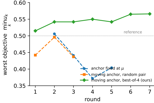
Figure 1: What the two design choices buy, on HELPSTEER2 under Qwen3-32B. Anchoring every round at the reference makes the weights chase whichever objective is currently worst against \mu , and the iteration gives back what it just repaired. Moving the anchor to the previous policy is not enough on its own: with a random pair of the anchor’s samples the round direction is too noisy and the swing persists. Selecting, among four samples, the pair with the largest weighted margin makes each round decisive, and the worst objective rises monotonically and stays above the reference.
