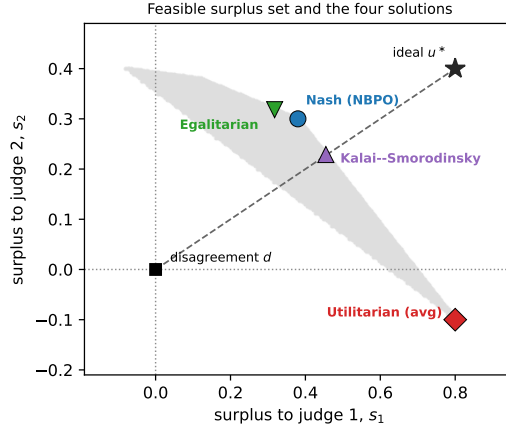
Figure 2: Feasible surplus set of a two-judge game (grey), with the disagreement point d at the origin and the ideal point u^* . The utilitarian (averaging) vertex leaves the positive orthant, driving judge 2 below the reference, while the Nash, Kalai–Smorodinsky, and egalitarian solutions stay strictly interior and distinct. Kalai–Smorodinsky lies on the dashed segment from d to u^* , as its definition requires.
