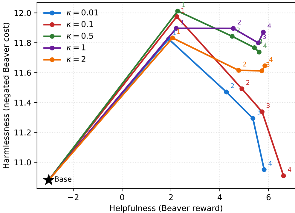
SafeRLHF RONPO trajectories by adversary temperature
