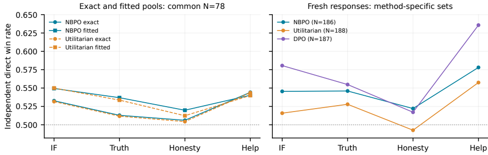
Figure 3: Descriptive reconstruction from Table 6. Left: exact and fitted-pool means on the same 78 prompts. Right: fresh-response means on method-specific sets (186/188/187 prompts for NBPO/utilitarian/DPO). Raw interval arrays were not supplied, so no error bars or unpaired difference estimates are reconstructed. The 0.5 line is the direct-win symmetry reference, not an estimated minimum-objective baseline.
