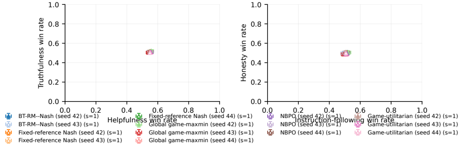
Figure 1: Empirical four-objective trade-offs: helpfulness versus truthfulness (left), and instruction following versus honesty (right). One point per evaluated policy seed rather than per method – 21 across the five mechanisms and the measured external baselines – on the 1,295 common prompts, with each seed’s own whole-prompt paired bootstrap interval. Seeds are plotted separately because a family mean has no defined prompt-bootstrap interval here: prompt uncertainty and seed spread are kept separate throughout and never pooled, and the scatter within a method is itself the panel’s main finding. Filled markers indicate descriptive dominance of point estimates over all four objectives among the plotted rows only; they do not imply significant dominance or population Pareto optimality. The base is the reference for every axis and sits at 0.5 by construction, so it is not plotted. Still pending, seven rows: Scalarized DPO (help heavy), Scalarized DPO (help only), Scalarized DPO (honesty only), Scalarized DPO (IF only), Scalarized DPO (truth heavy), Scalarized DPO (truth only) and PROSPER (adapt.).
