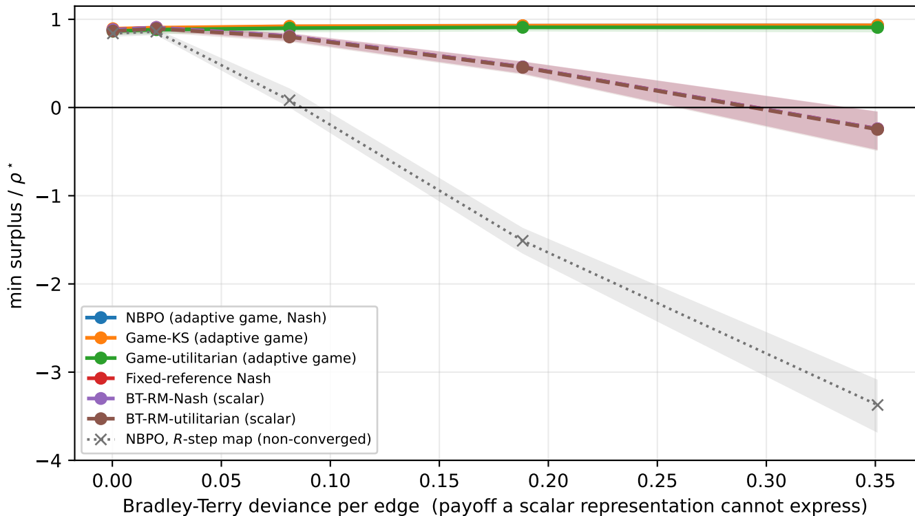
Feasibility-preserving controlled nontransitivity ( \rho^* held fixed)
