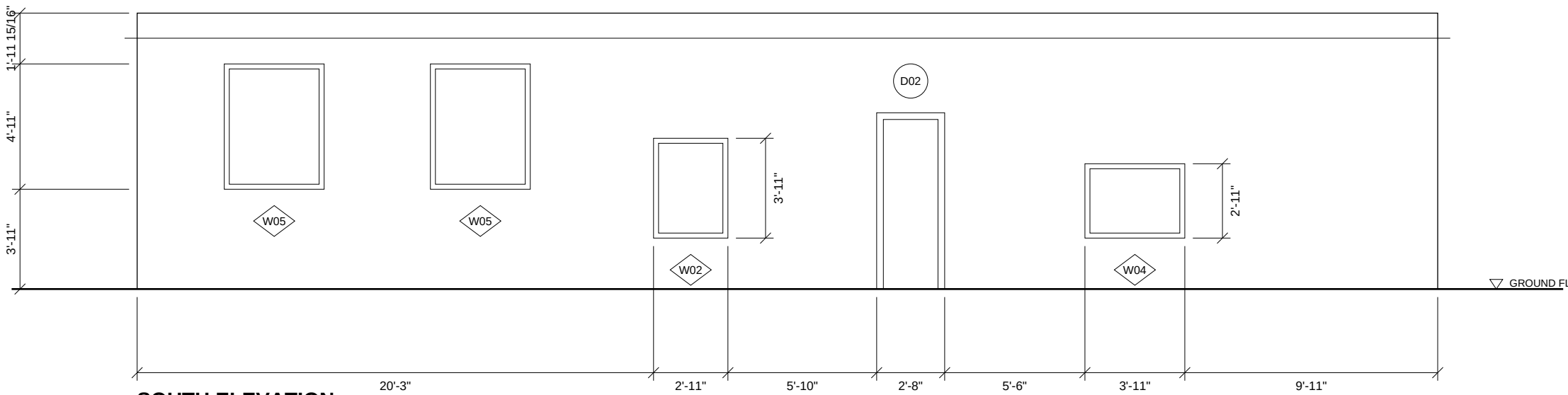
SOUTH ELEVATION
