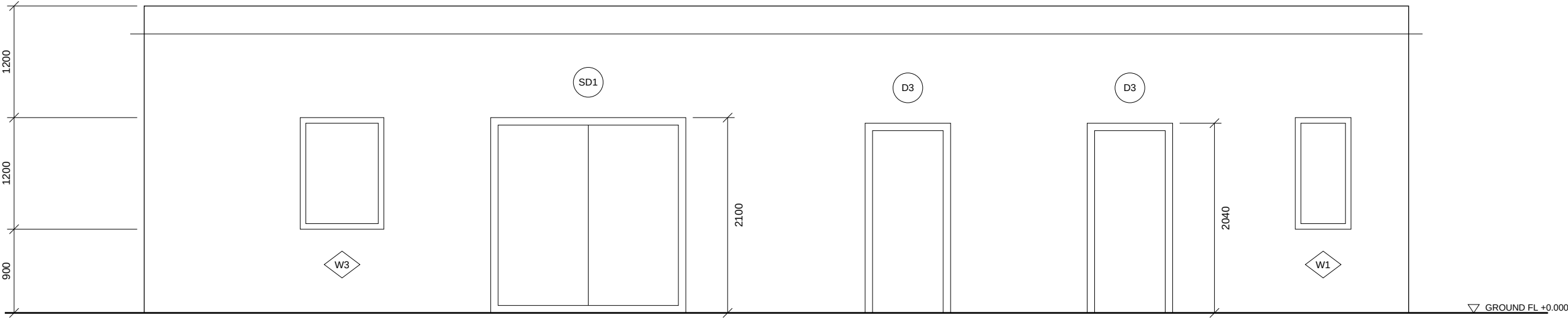
NORTH ELEVATION
