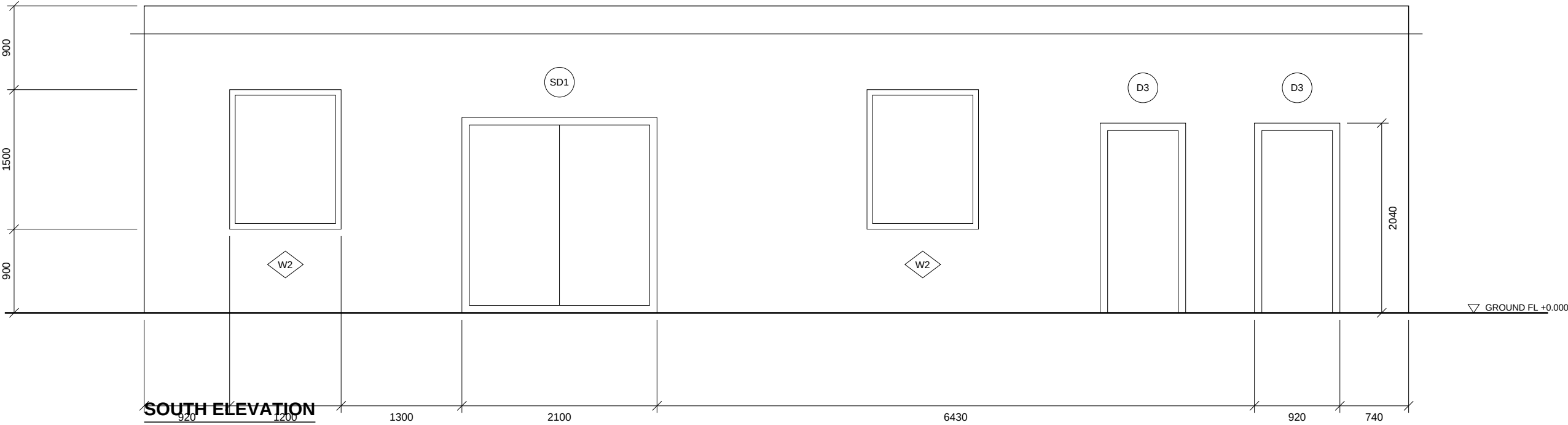
SOUTH ELEVATION
