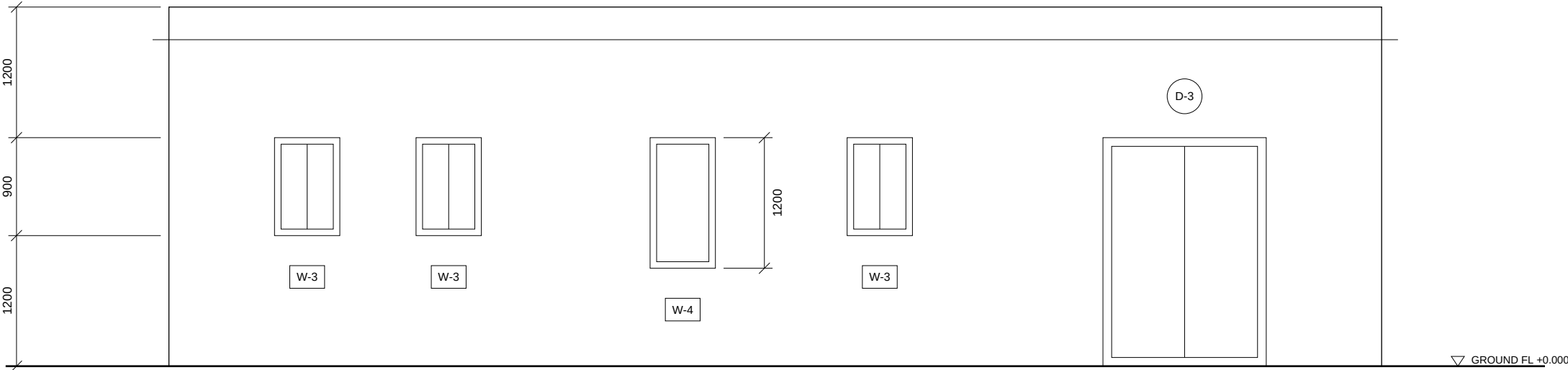
NORTH ELEVATION
