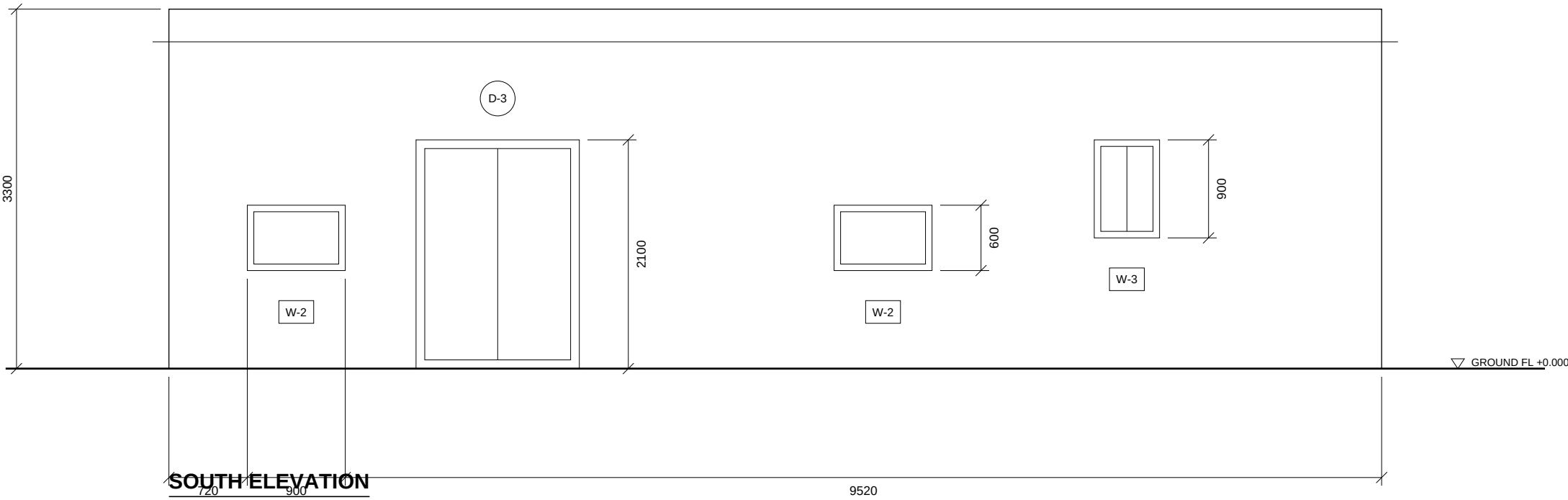
SOUTH ELEVATION
