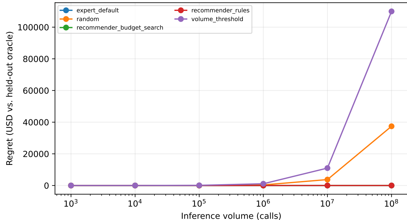
Deployment regret vs. volume: banking77
