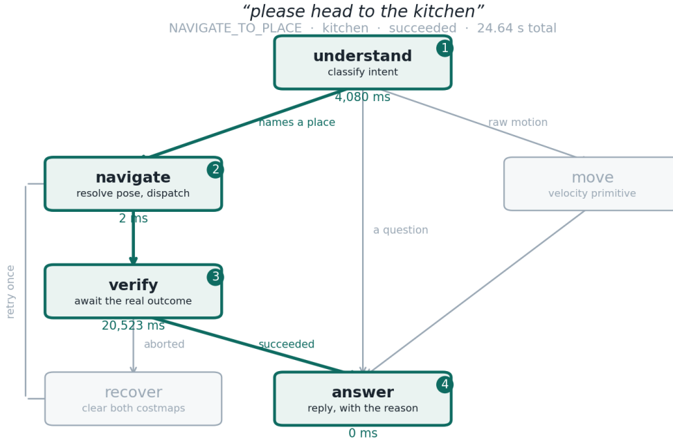
Figure 3.7. A recorded command traced through the policy. Nodes and edges the run touched are highlighted, numbered in execution order, and annotated with the time each node held the command. Almost the whole 24.64 s is spent in verify waiting for the navigation outcome; intent parsing takes 4.08 s and the remaining nodes are effectively instantaneous. Drawn by scripts/plot_trace.py from the policy’s own trace log.
