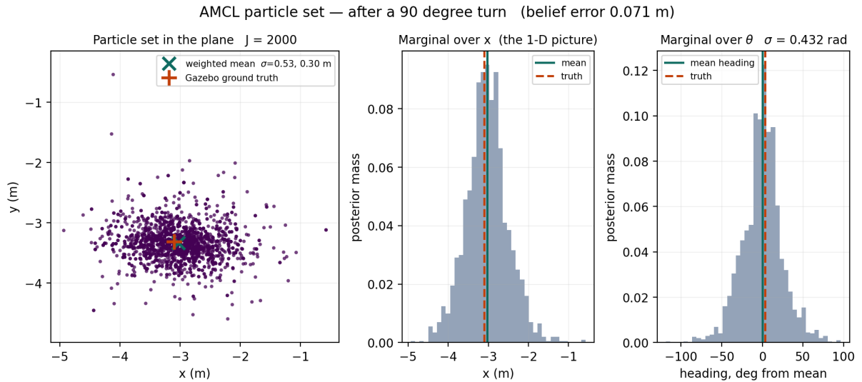
Figure 3.11. The same set after a 90^\circ rotation, with the corrected motion-noise coefficients of Listing 3.2. Heading spread is 0.432 rad against 0.481 rad before the turn, and belief error is 0.071 m. Under the coefficients used before correction the same manoeuvre multiplied heading spread by 9.3 (Table 4.6).
