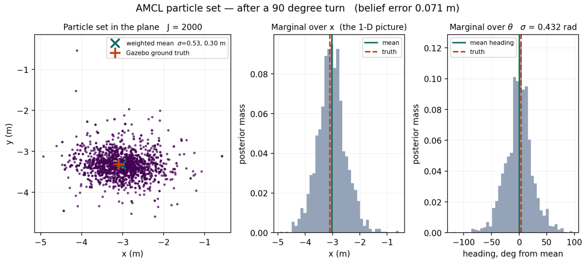
Figure 3.13. The same set after a 90° rotation, with the corrected motion-noise coefficients of Listing 3.2. Heading spread is 0.432 rad against 0.481 rad before the turn, and belief error is 0.071 m. Under the coefficients used before correction the same manoeuvre multiplied heading spread by 9.3 (Table 4.6).
