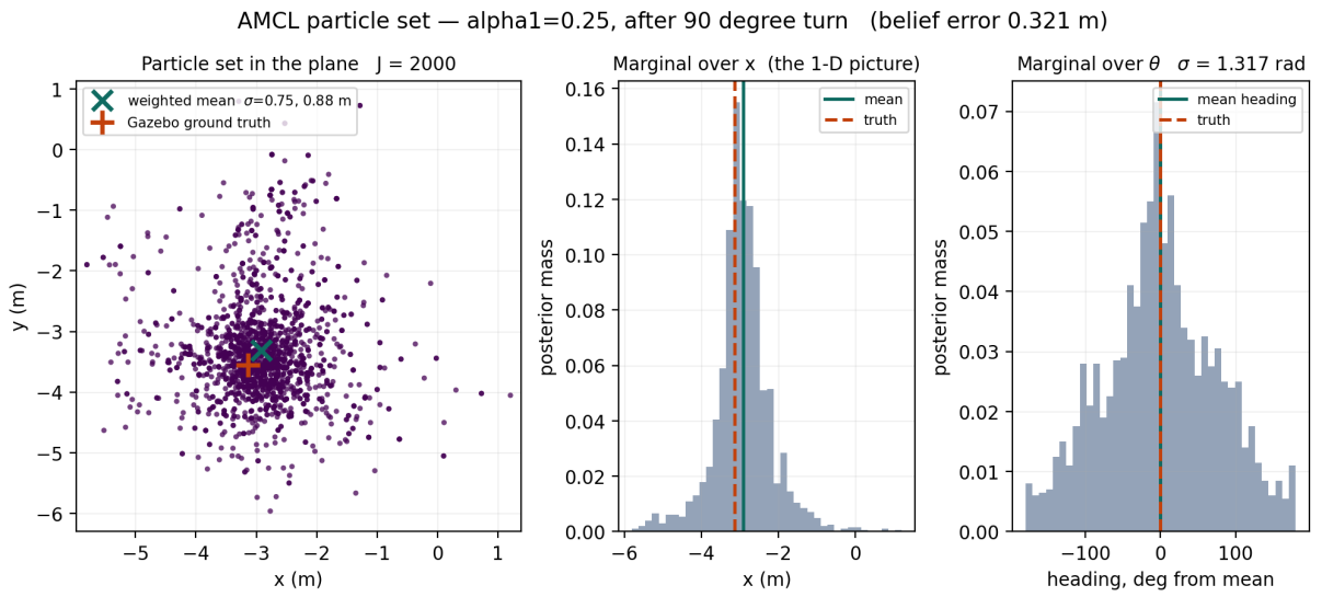
Figure 3.14. The particle set after the same 90° rotation with \alpha_1 = \alpha_2 = 0.25 . The cloud spans several metres and the heading marginal carries mass across the entire circle: the robot has no useful estimate of which way it is facing. Compare Figure 3.13, the identical manoeuvre at \alpha_1 = 0.02 .
