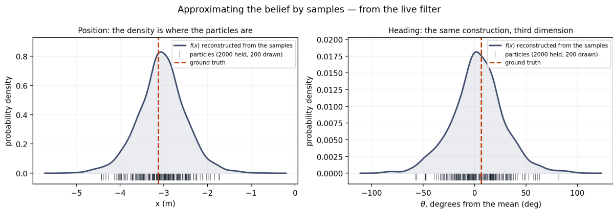
Figure 3.11. The belief as an approximation by samples, captured from the running filter. Each tick is one particle; the curve is reconstructed from the ticks rather than stored. Left, the marginal over x ; right, the marginal over heading. Because the filter resamples on every update, all 2000 particles carried identical weight, so the probability of a region is expressed by how many samples fall in it.
