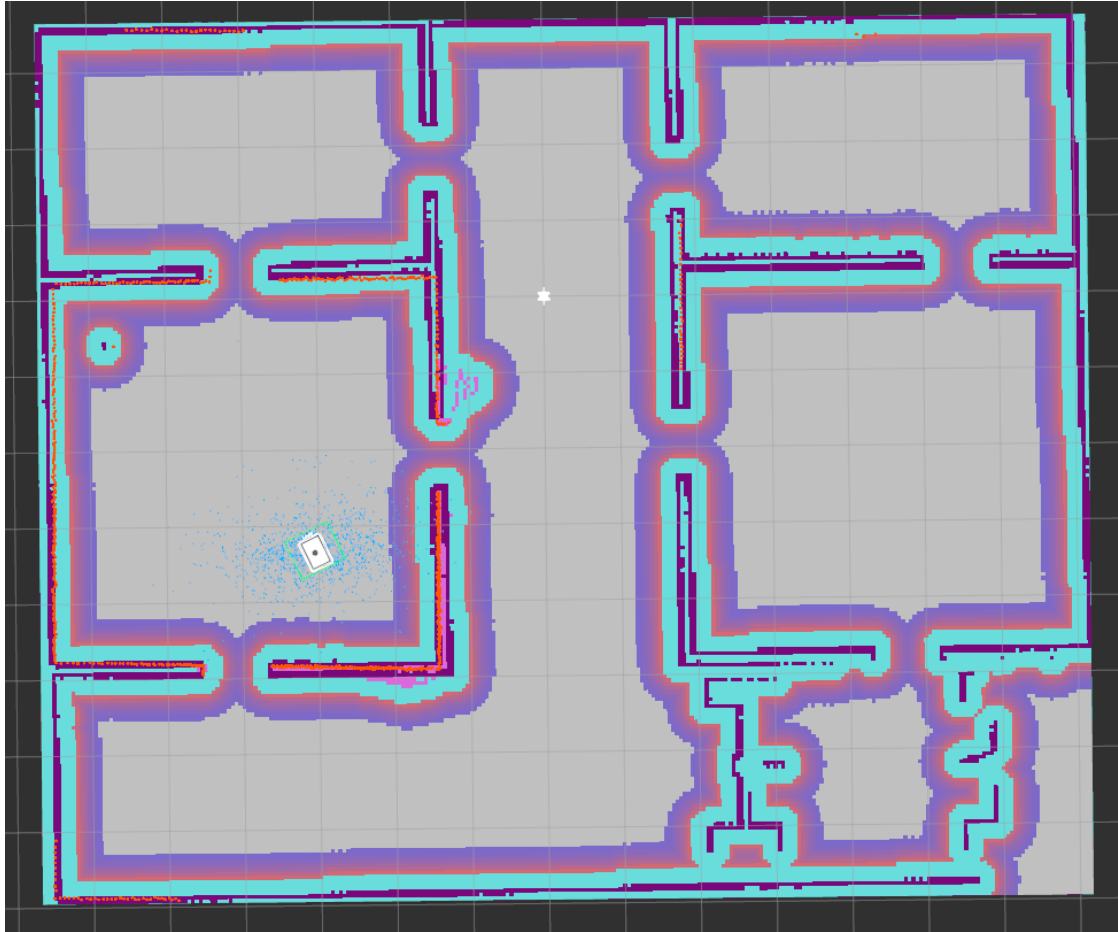
Figure 3.10. The navigation subsystem in operation, with the robot spawned and AMCL active. Grey is free space in the static map. The cyan band hugging each wall is the region within the robot’s inscribed radius, which the planner treats as blocked; the purple gradient outside it is the inflation layer, whose cost decays with distance and steers paths toward the middle of a corridor rather than along its edge. Orange points are live laser returns, lying on the mapped walls — the agreement quantified in Section 4.4. At the left of the plan the robot’s footprint is drawn as the rectangular polygon it is modelled by, rather than a circumscribing circle, surrounded by the blue particle cloud: the same sample set plotted analytically in Figures 3.12–3.14, here shown in place. The extent of that cloud relative to the rooms around it is the robot’s uncertainty about which part of the building it occupies.
