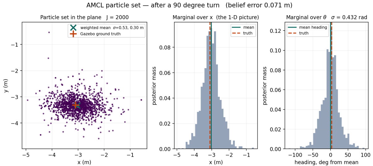
Figure 3.13. The same set after a 90^\circ rotation, with the corrected motion-noise coefficients of Listing 3.2. Heading spread is 0.432 rad against 0.481 rad before the turn, and belief error is 0.071 m. Under the coefficients used before correction the same manoeuvre multiplied heading spread by 9.3 (Table 4.6).
