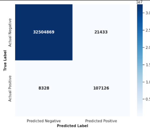
Fig. 3. Global pixel-level confusion matrix. This matrix illustrates the model’s predictive performance where diagonal elements denote correct classifications (TN and TP) and off-diagonal elements indicate misclassifications (FP and FN). This study includes this visualization to demonstrate that despite severe class imbalance, the model achieves a remarkably low False Positive Rate of 6.6 \times 10^{-4} , confirming its high specificity in distinguishing healthy tissue while successfully capturing critical lesion areas.
