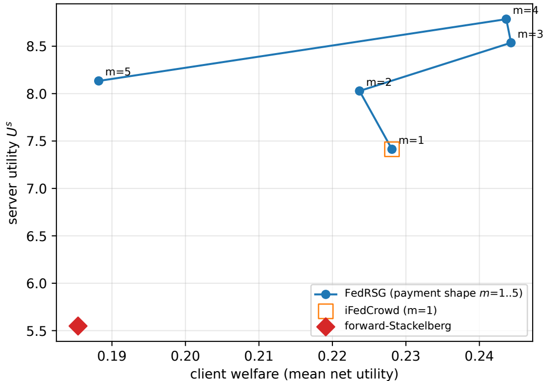
mnist: measured-oracle frontier
