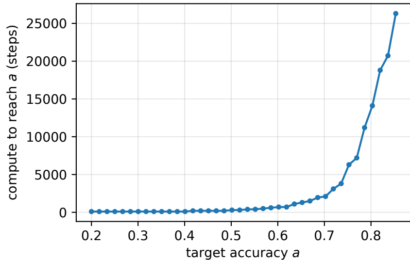
cifar10: C^{comp}(a)
