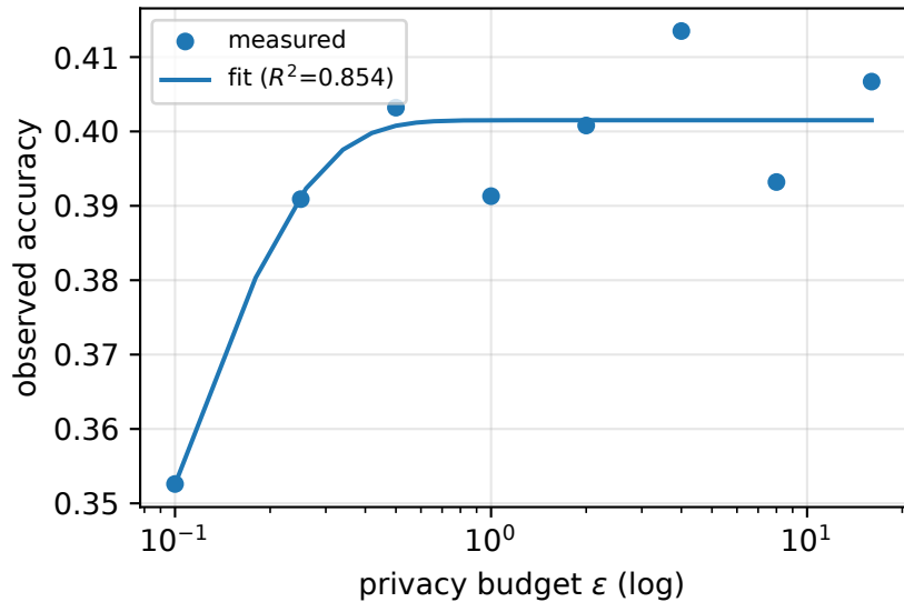
cifar10: A(a, \epsilon)
