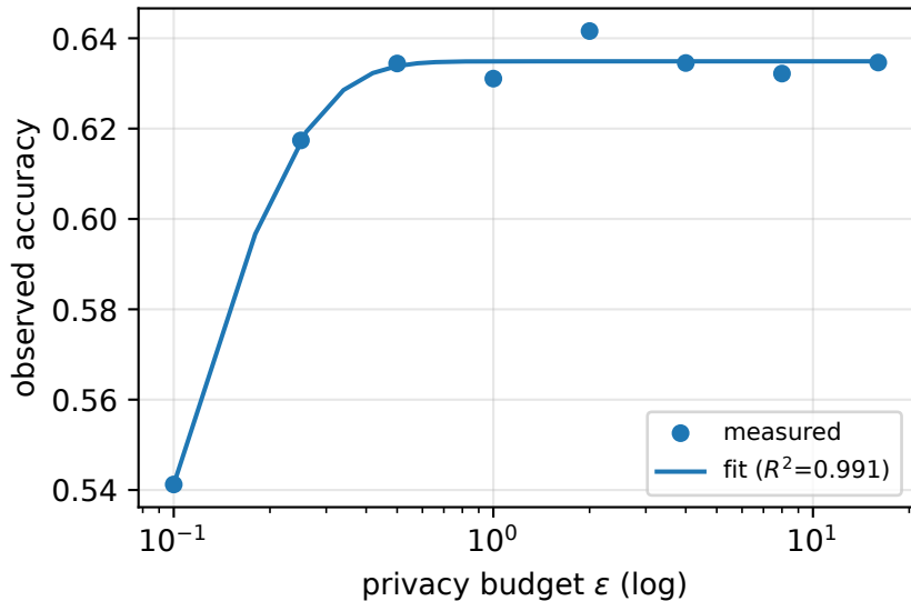
femnist: A(a, \epsilon)
