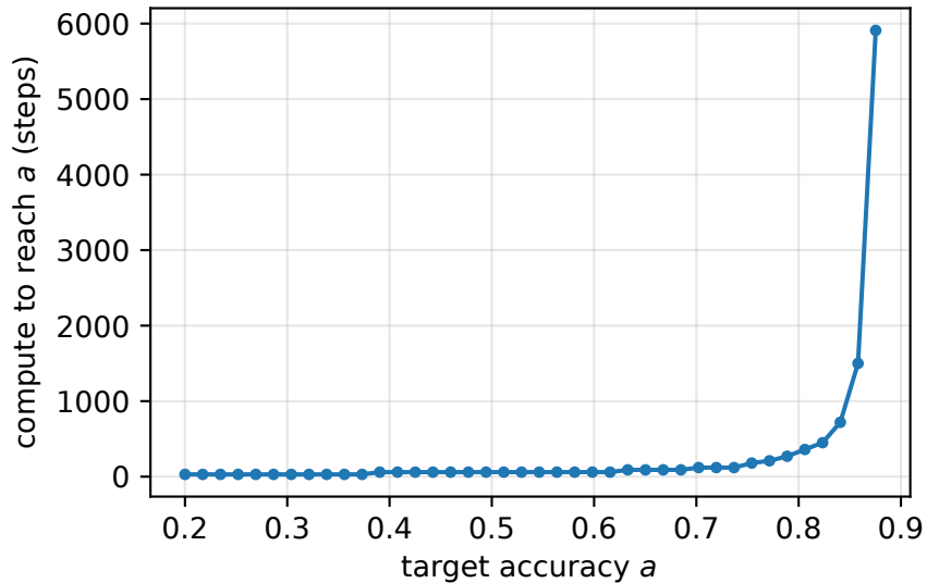
femnist: C^{comp}(a)
