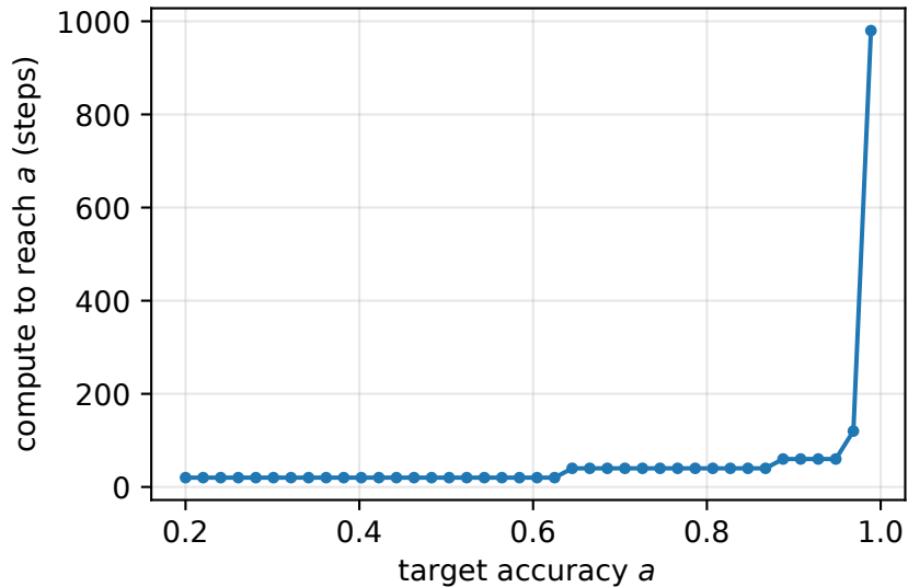
mnist: C^{comp}(a)
