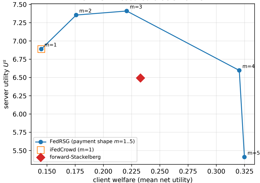
femnist: measured-oracle frontier
